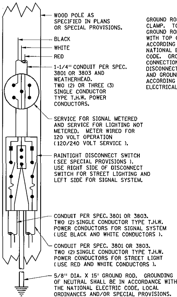
METER AND DISCONNECT SWITCH WIRING DIAGRAMS
