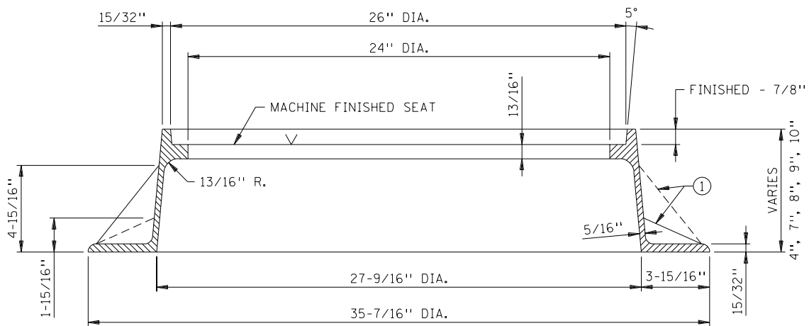
SECTION A-A (NO. 700-7 SHOWN)
