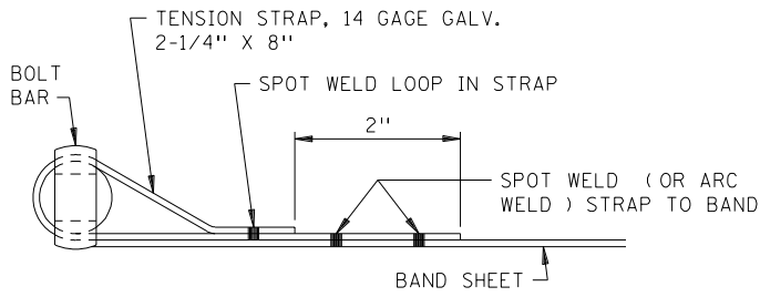
STRAP STRAP DETAIL
