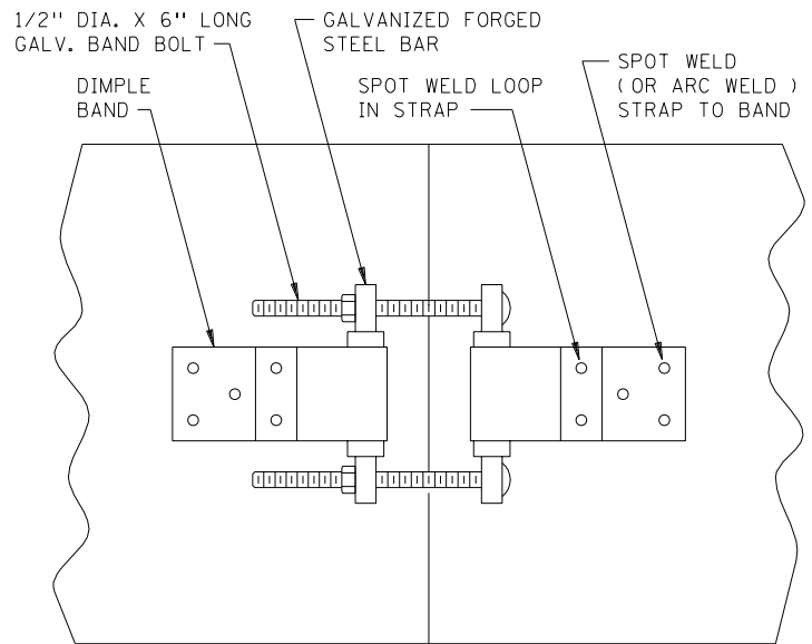
BAR AND STRAP CONNECTION
