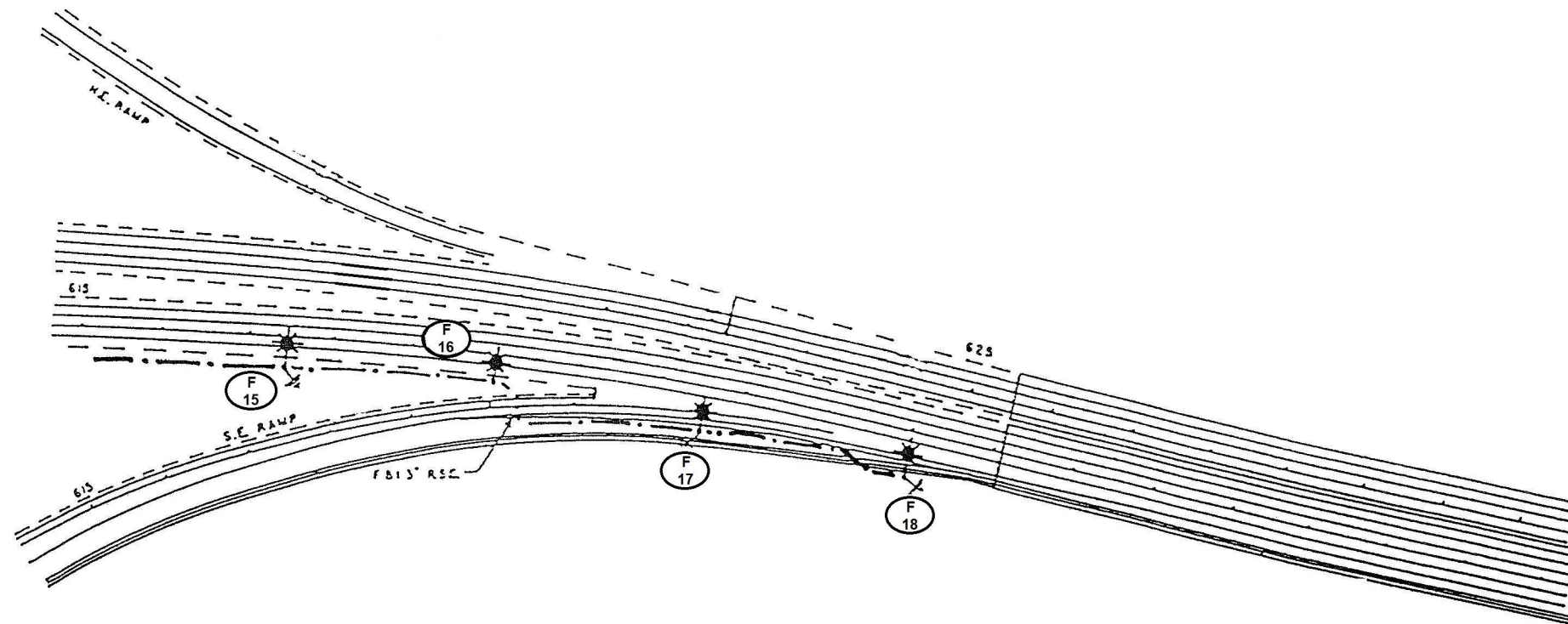
FEEDPOINT A00F LIGHTING STANDARDS AND FOUNDATIONS
