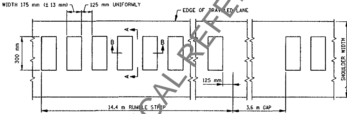
PLAN VIEW B - Type 2 INTERMITTENT PATTERN
