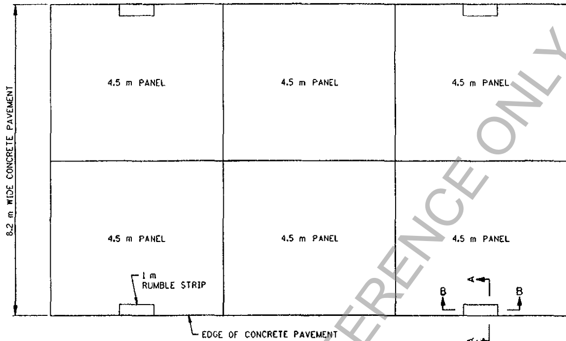
PLAN VIEW - Type 4
