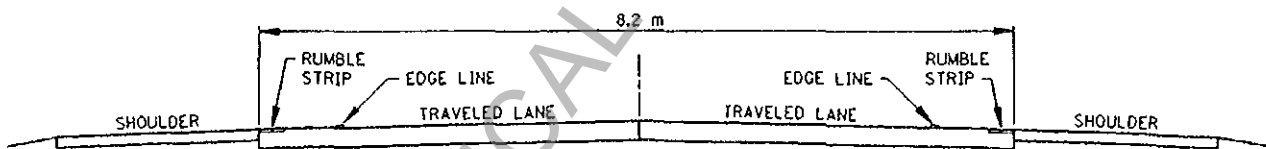
SECTION VIEW OF ROADWAY
