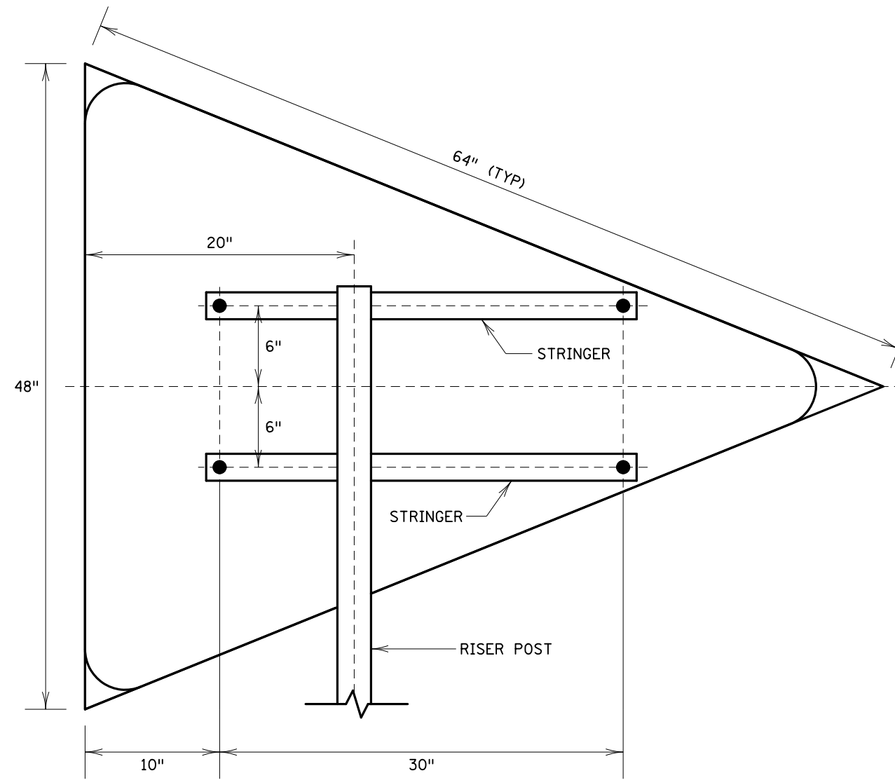
NO PASSING ZONE MOUNTING DETAIL
