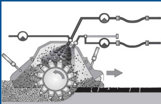
(Above): Diagram of the full depth recycling process
