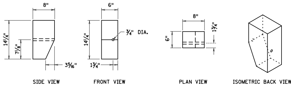
SIDE VIEW FRONT VIEW PLAN VIEW ISOMETRIC BACK VIEW 6" x 8" x 14 1/4" TAPERED WITH SINGLE OFFSET POST BOLT HOLE
