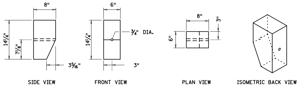
SIDE VIEW FRONT VIEW PLAN VIEW ISOMETRIC BACK VIEW 6" x 8" x 14 1/4" TAPERED WITH SINGLE CENTERED POST BOLT HOLE
