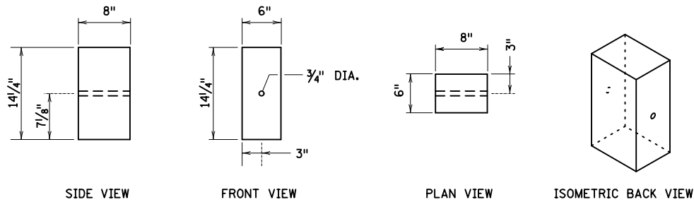
SIDE VIEW FRONT VIEW PLAN VIEW ISOMETRIC BACK VIEW 6" x 8" x 14 1/4" SINGLE CENTERED POST BOLT HOLE
