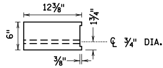
PLAN VIEW
