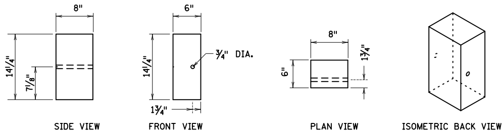
SIDE VIEW FRONT VIEW PLAN VIEW ISOMETRIC BACK VIEW 6" x 8" x 14 1/4" WITH SINGLE OFFSET POST BOLT HOLE
