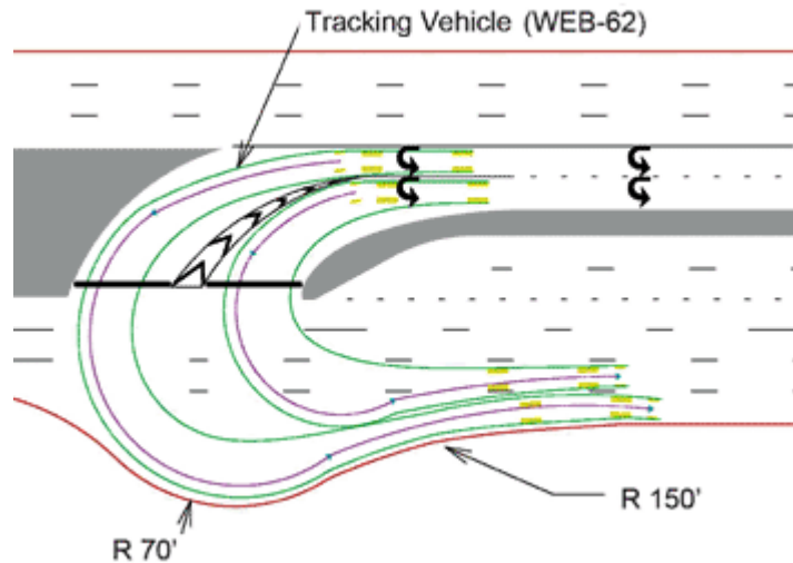
Figure 2- loon at a crossover Source: FHWA, 2009a
