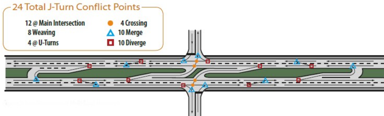
Figure 1: J-turn Intersection Source: FHWA, 2009
