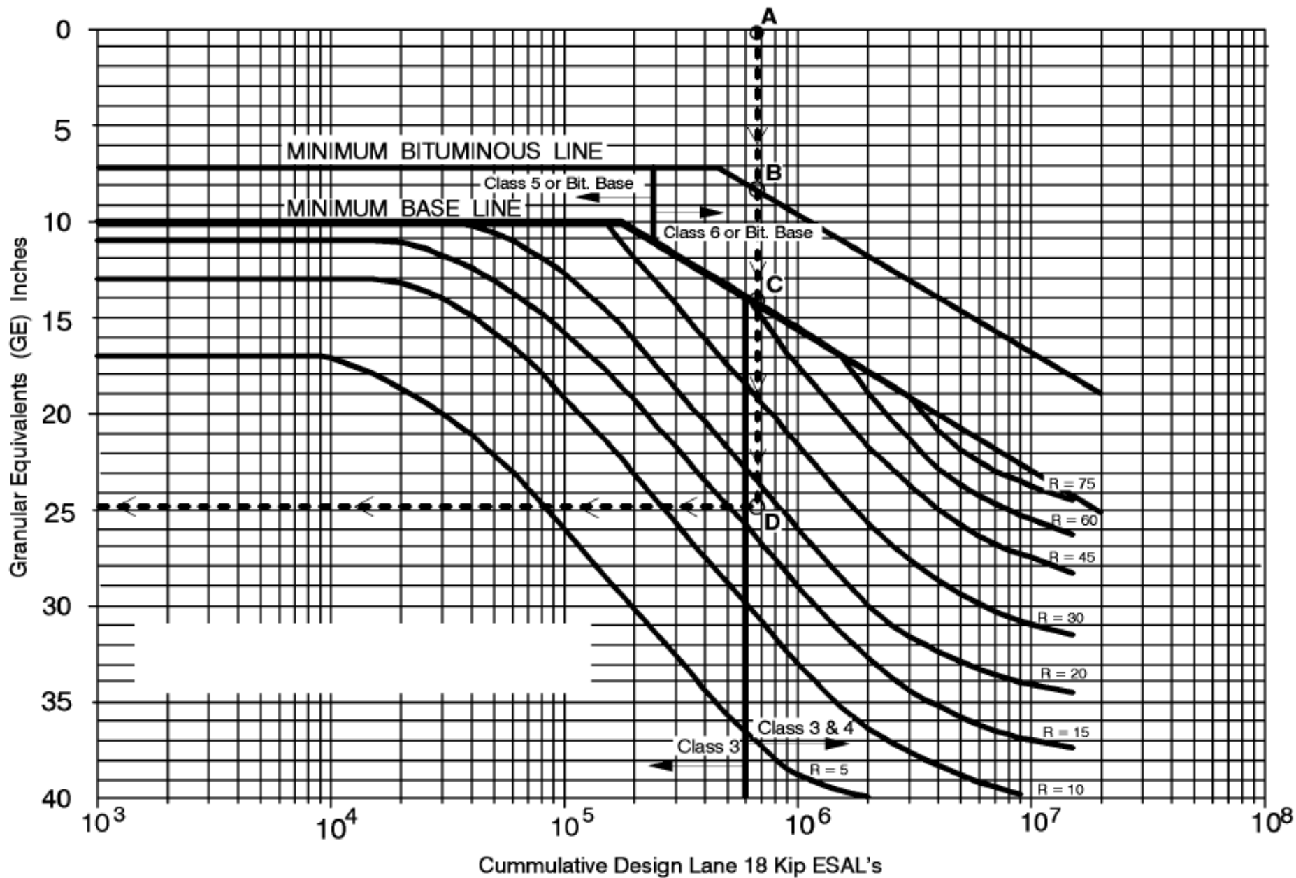
BITUMINOUS PAVEMENT DESIGN CHART (AGGREGATE BASE)
