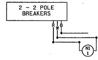
FEEDPOINT 19N1 LIGHTING UNIT LOCATION AND TYPE
