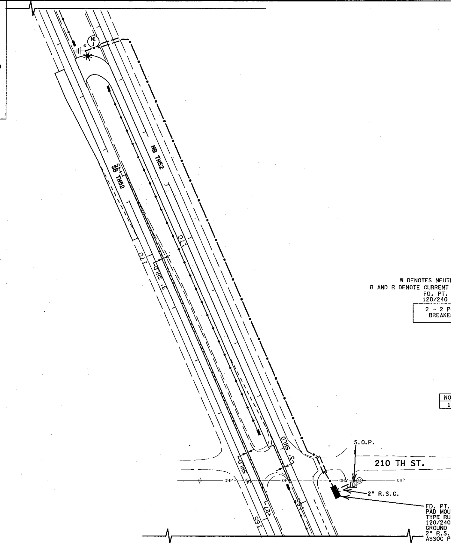
FEEDPOINT 19N1 LIGHTING UNIT LOCATION AND TYPE
