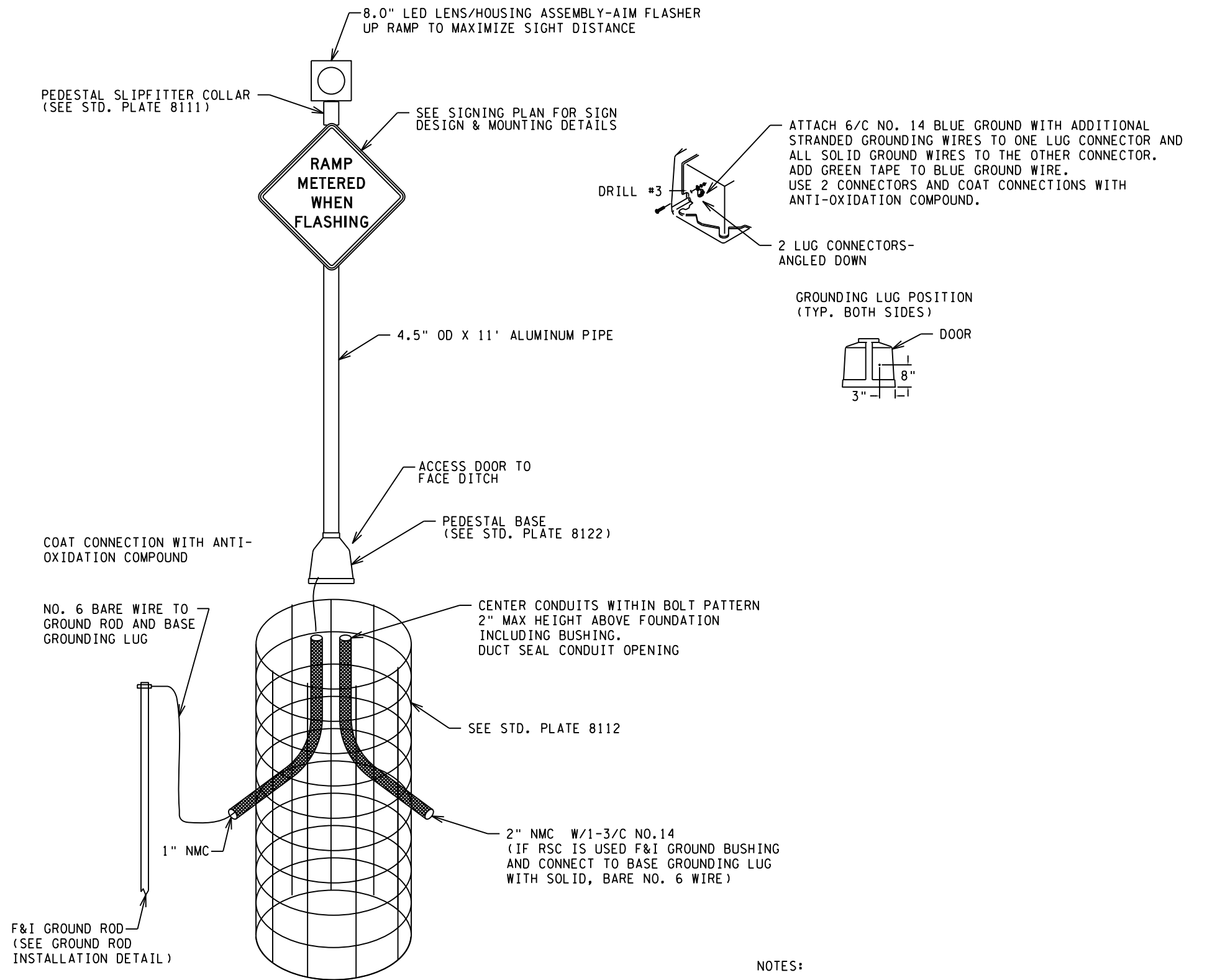
FLASHER DETAIL
