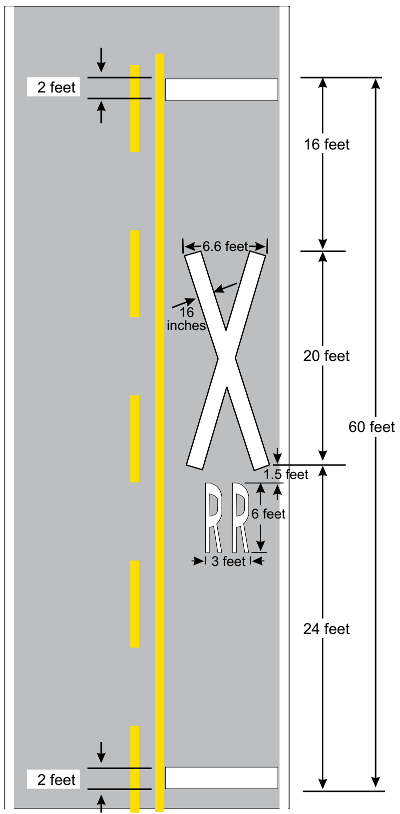
Figure 8B-7 Grade Crossing Pavement Markings
