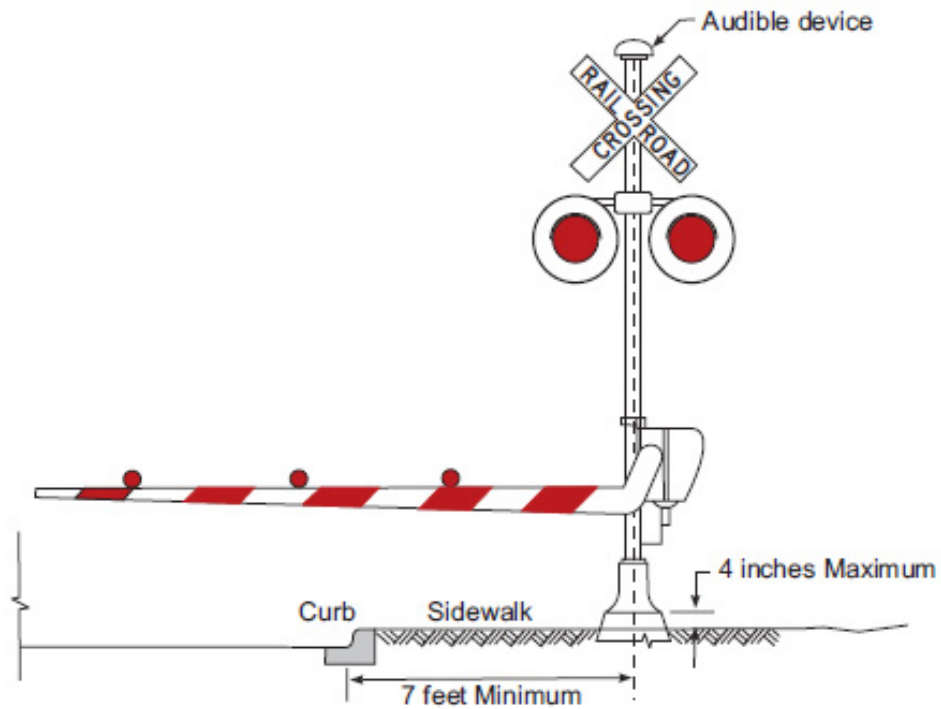
Figure 8C-5 Example of a Shared Pedestrian/Roadway Gate
