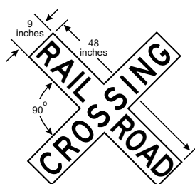
R15-1 Drilled for 90-degree mounting
