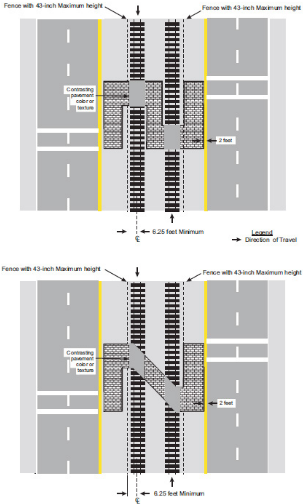
Figure 8C-10 Examples of Pedestrian Barrier Installation at an Offset Non-Intersection Grade Crossing
