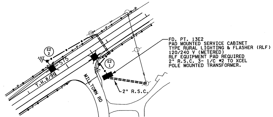
FEEDPOINT 13E2 LIGHTING STANDARDS AND FOUNDATIONS
