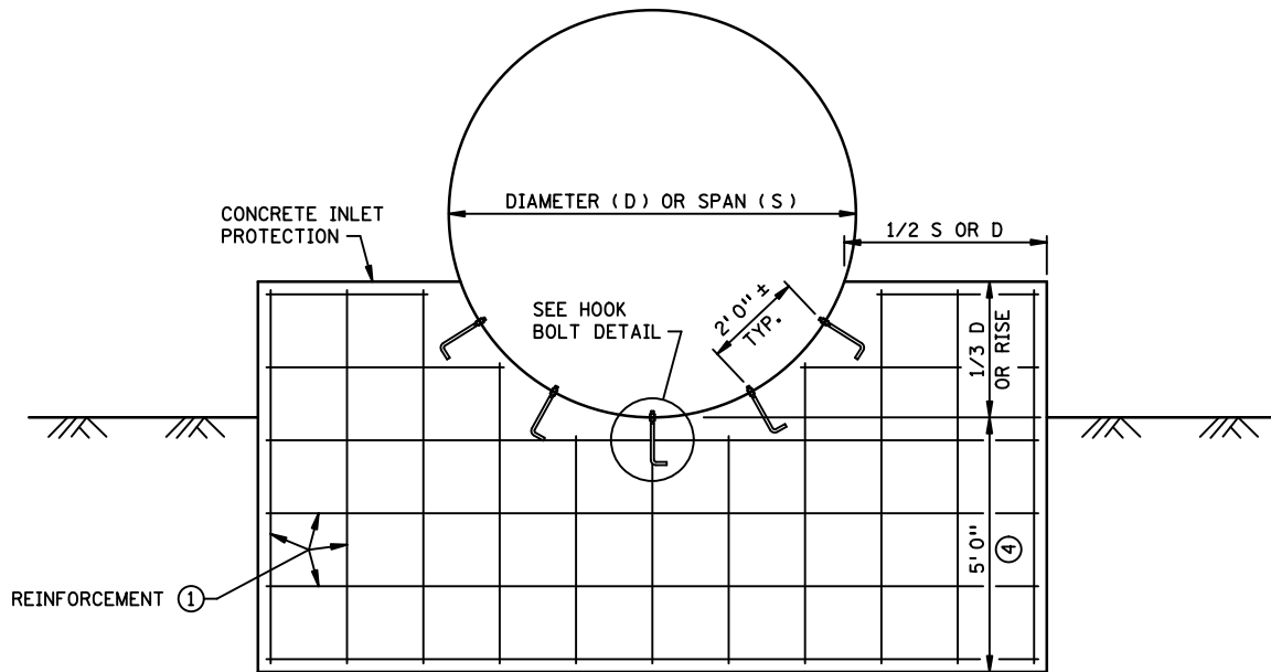
FRONT VIEW
