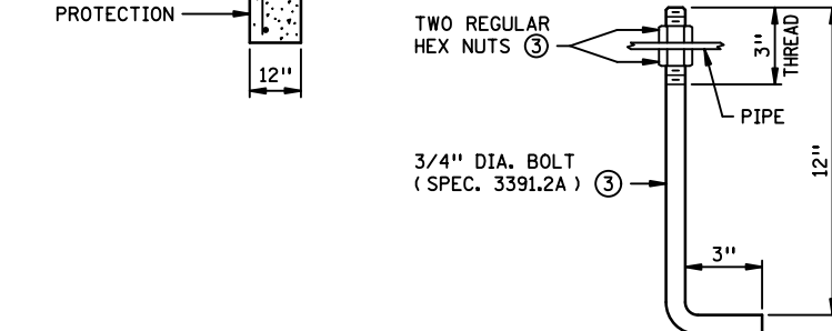
HOOK BOLT
