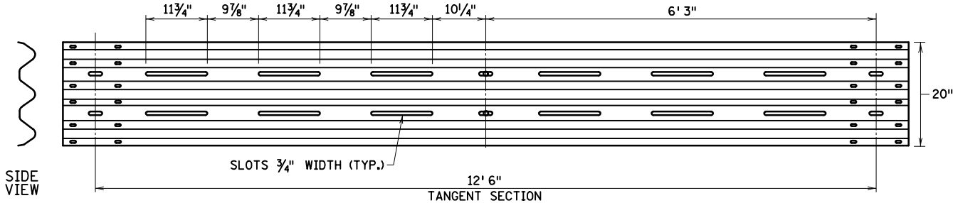
FRONT VIEW SLOTTED RAIL NO. 3
