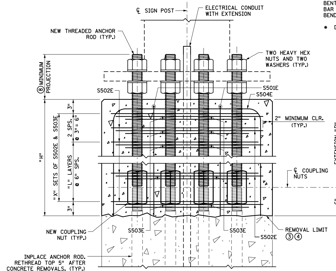
SECTION A-A INPLACE REINFORCEMENT NOT SHOWN FOR CLARITY
