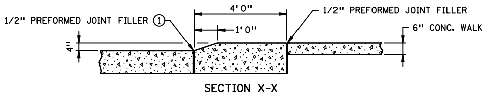
SECTION X-X
